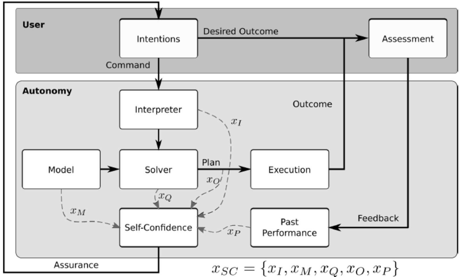
Factorized Machine Self-Confidence
